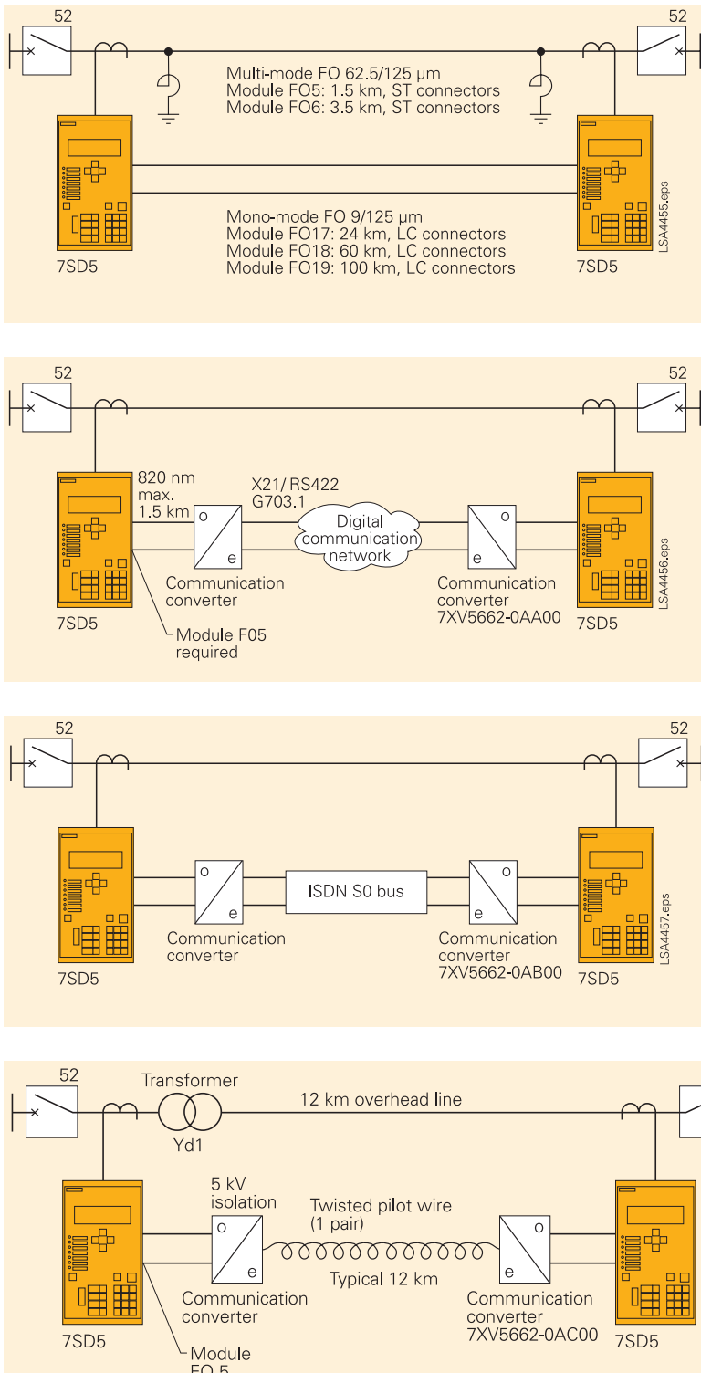
Fig.12 Examples for communication links
