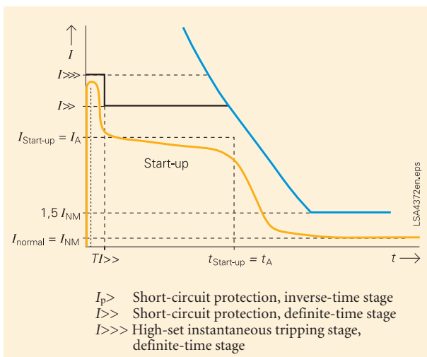
Fig. 5 Current characteristic of motor start-up
