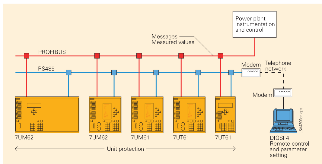
Fig. 7 Integration of protection relays into power station control and protection system
